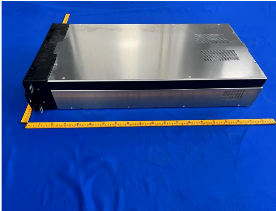
样品图片,内部电池模块 (Sample photograph, internal battery module) -19
